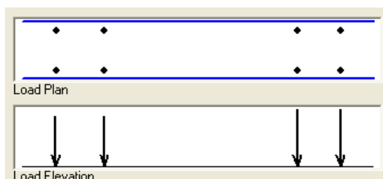
Figura 3.2 – Veículo ONIB-DD-TRUC (4CB) – ( E_1 a E_2 )=64,5 kN / ( E_3 a E_4 )=72,5 kN / d_{12}=1,45 m / d_{23}=5,82 m / d_{34}=1,30 m
