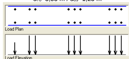
Figura 3.5 – Veículo BT-74/25 (3Q6) – E_1=57,0 \text{ kN} / ( E_2 \text{ a } E_9=90,0 \text{ kN} / d_{12}=3,06 \text{ m} / d_{23}=1,25 \text{ m} / d_{34}=7,03 \text{ m} / d_{45}=1,25 \text{ m} / d_{56}=1,25 \text{ m} / d_{67}=6,15 \text{ m} / d_{78}=1,25 \text{ m} / d_{89}=1,25 \text{ m}
