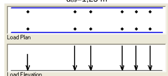
Figura 3.6 – Veículo BB-48/14 (3J3) – E_1=60,0 \text{ kN} / ( E_2 \text{ a } E_6=90,0 \text{ kN} / d_{12}=4,20 \text{ m} / d_{23}=1,40 \text{ m} / d_{34}=2,80 \text{ m} / d_{45}=1,25 \text{ m} / d_{56}=1,25 \text{ m}
