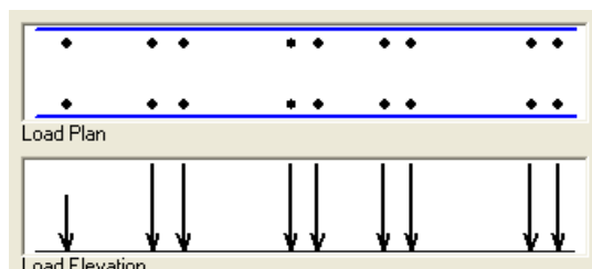
Figura 3.4 – Veículo RT-74/25 (3T6-b) – E_1=57,0 \text{ kN} / ( E_2 \text{ a } E_9=90,0 \text{ kN} / d_{12}=3,975 \text{ m} / d_{23}=1,45 \text{ m} / d_{34}=4,95 \text{ m} / d_{45}=1,25 \text{ m} / d_{56}=3,05 \text{ m} / d_{67}=1,25 \text{ m} / d_{78}=5,55 \text{ m} / d_{89}=1,25 \text{ m}
